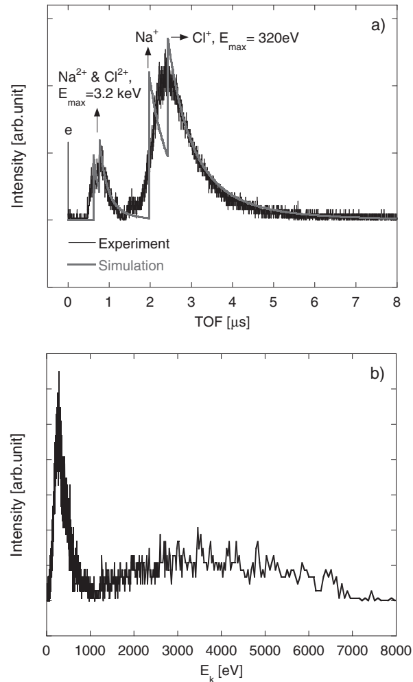
Fig. 8. (a) A model prediction of mass spectrum obtained in a field-free condition. (b) Kinetic energy distribution transformed on the basis of Na.
