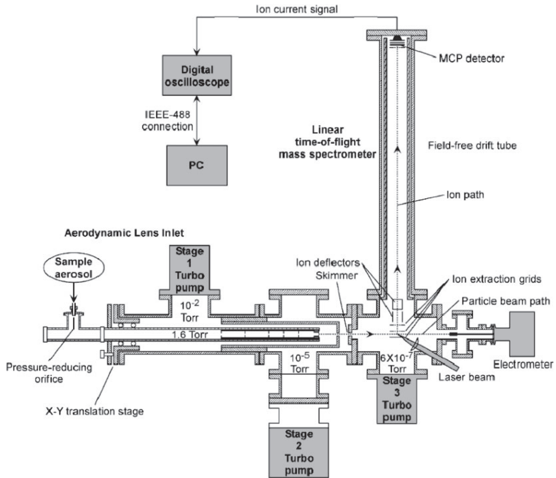
Fig. 1. Schematic of single particle mass spectrometry.
