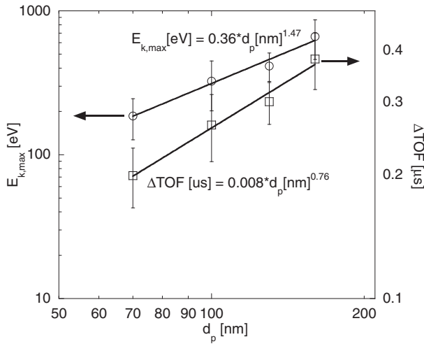
Fig. 3. Power dependences of maximum kinetic energy and difference in TOF on the particle size.
