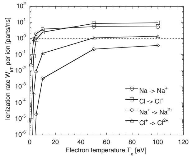
Fig. 4. Collision ionization rate of ions and atoms at solid density for 70 nm NaCl particle.
