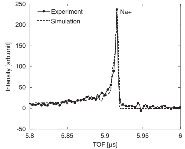
Fig. 6. Simulation of mass spectral peak profile of sodium ion from a 70 nm NaCl particle.
