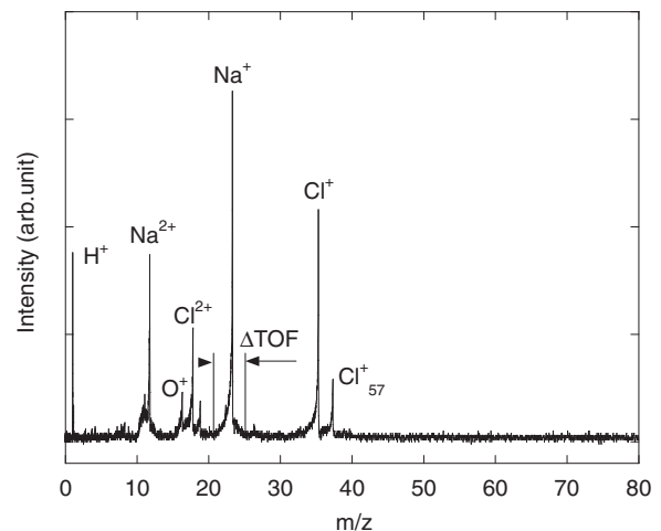
Fig. 2. Typical mass spectrum of a 70 nm NaCl nanoparticle.
